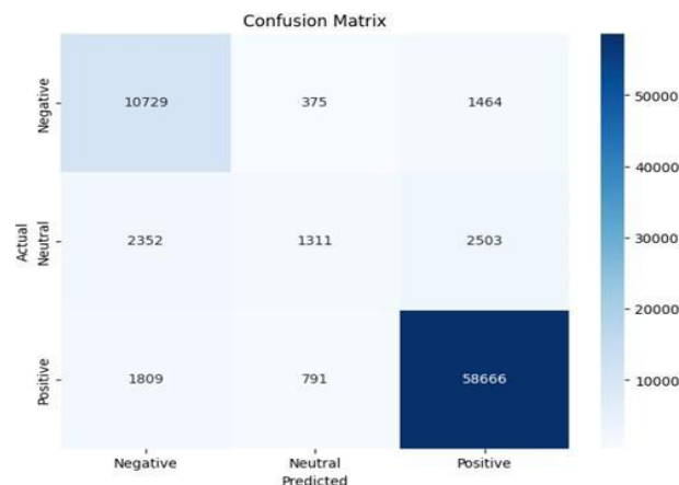
Fig. Confusion Matrix For BERT
