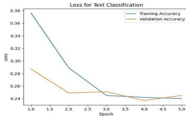
Fig. Training and Validation Loss for BERT
