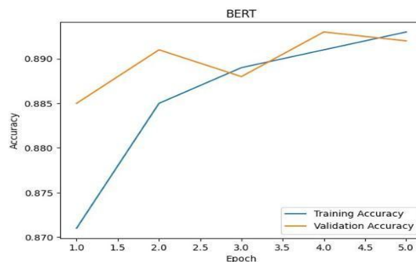
Fig. Training and Validation Accuracy for BERT
