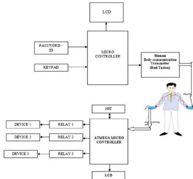
Fig1: A block diagram of a high-security framework using RedTacton technology
