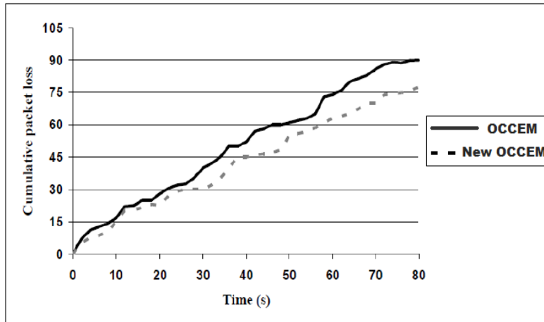
Figure 4. Cumulative Packet Loss
